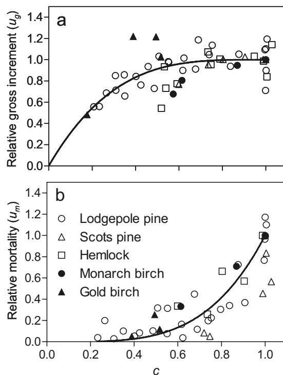
Figure 4. Relative gross stem-wood increment (a) and mortality (b) as functions of closure ( c ). Solid lined are best fits for all species pooled (see Tab. II). One point for Scots pine was outside of the plotted range (relative mortality = 2.14, c = 0.95 ).
